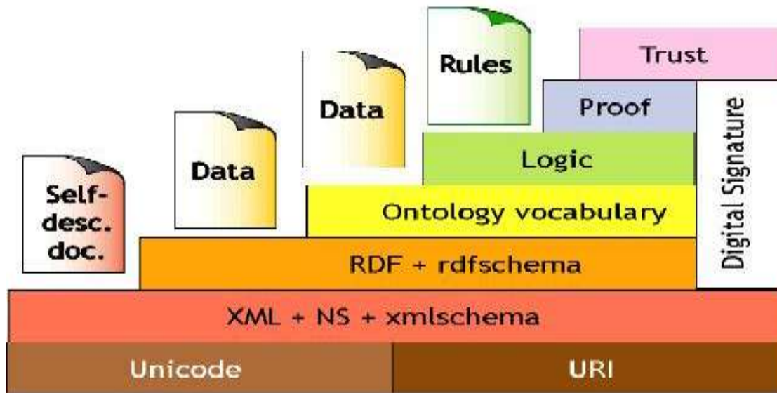
Figure 1 : Layer structure of semantic web [3]
