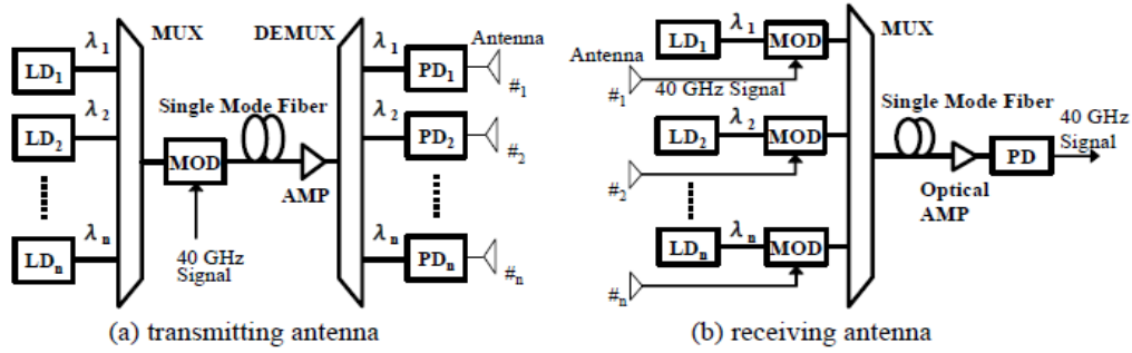
Figure 1: Schematic diagram of WDM-based optically controlled array antenna.
