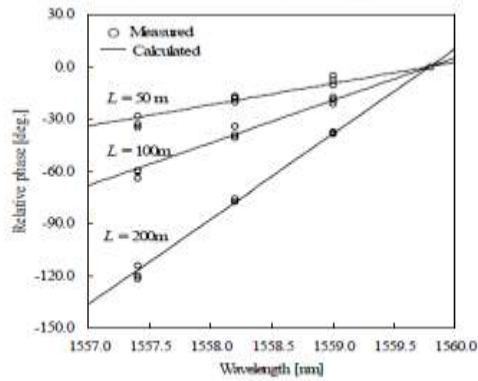
Figure 3: Measured 40 GHz phases at SMF length L = 50, 100 and 200 m.
