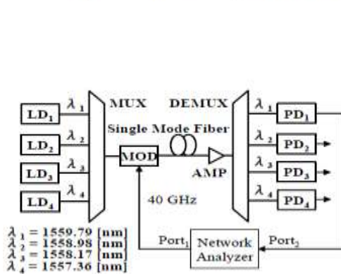
Figure 2: Experimental setup of 4-element optically controlled array antenna.
