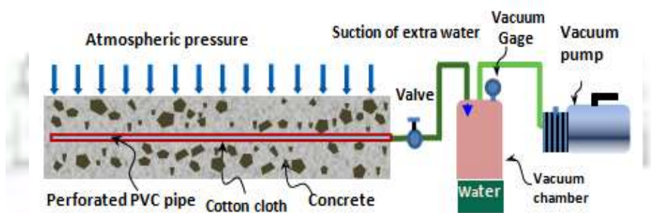
Figure (2) diagrammatic representation for new vacuum dewatering technique
