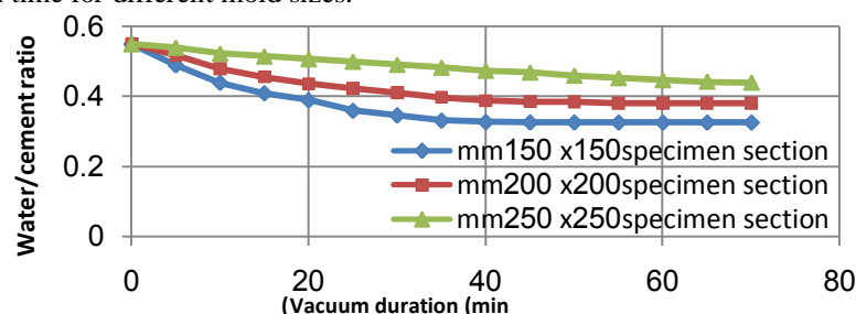
Figure (4) Relation between water/cement ratio and vacuum duration
