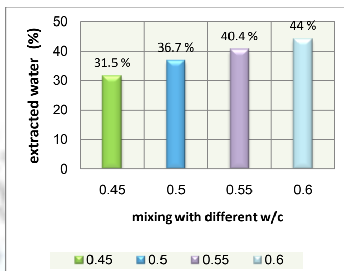
Figure (5): relation between water/cement ratio and extracted water
