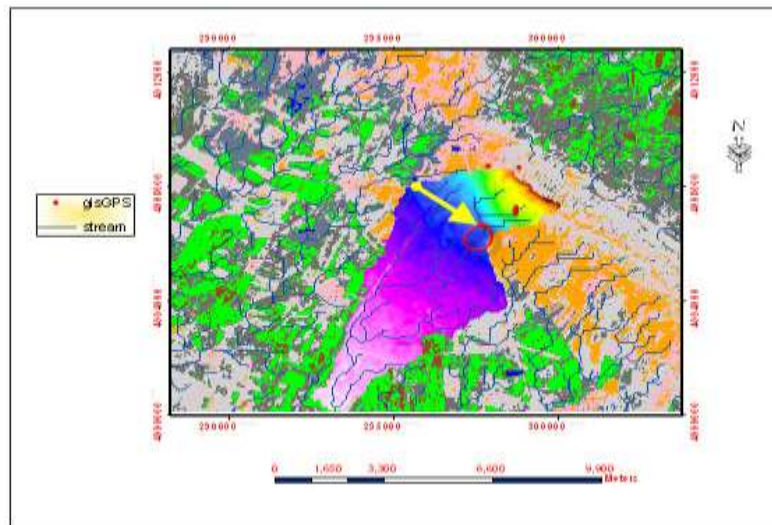
Figure (15): Suggested dam or barrier in Addaya site
