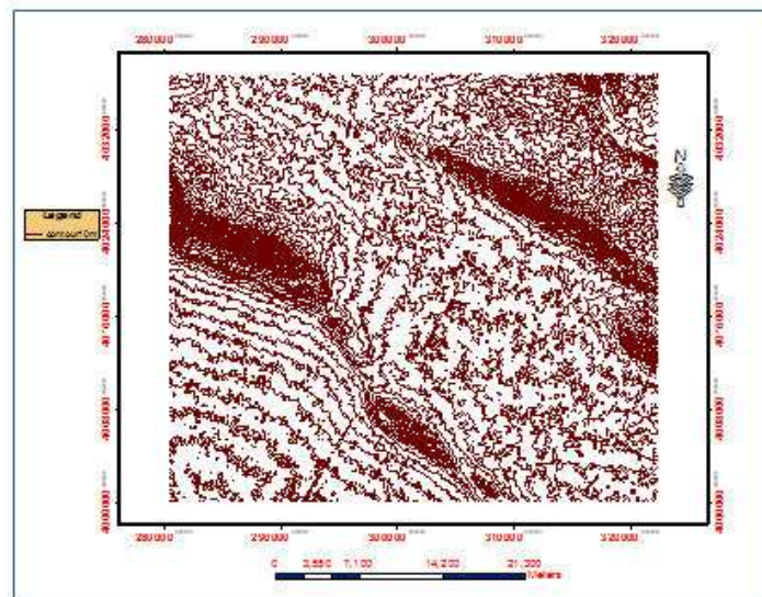
Figure (6): contour map of (10m) interval
