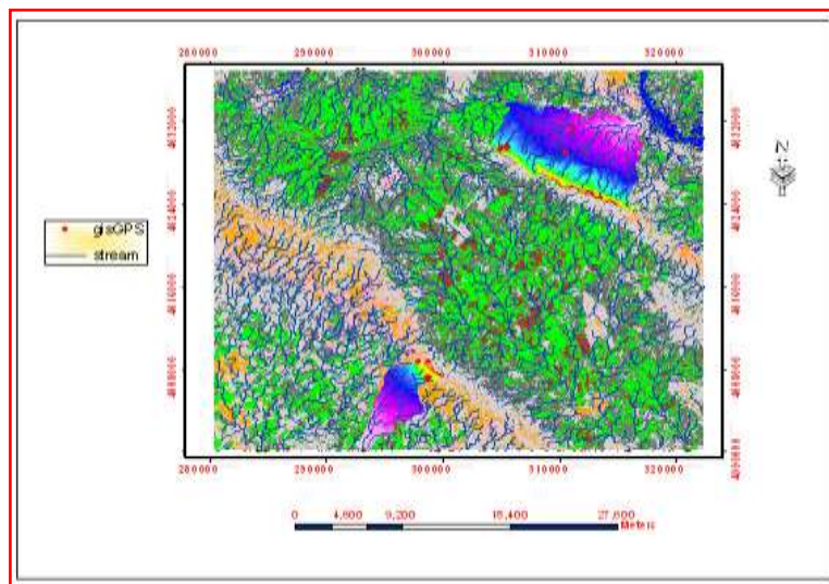
Figure (13): The catchment areas and the drainage patterns of the two sites
