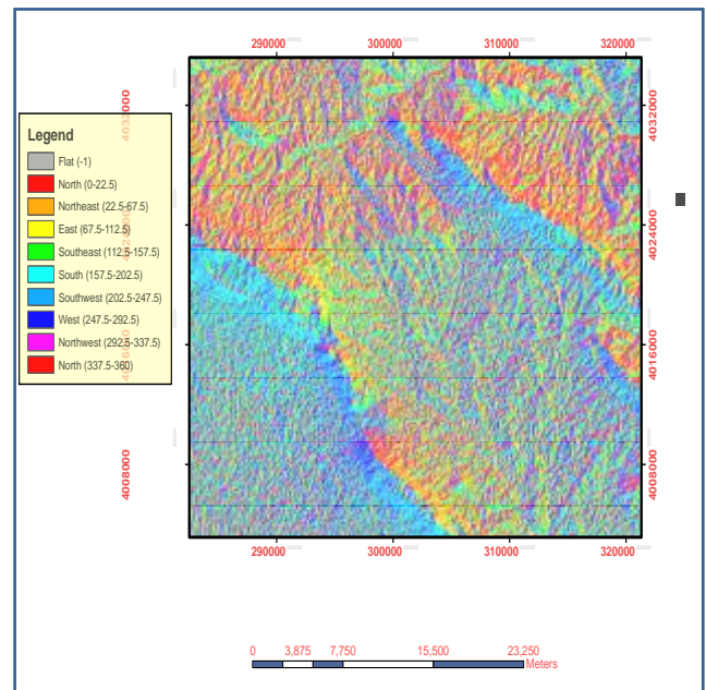
Figure (8): Aspect map of the study area
