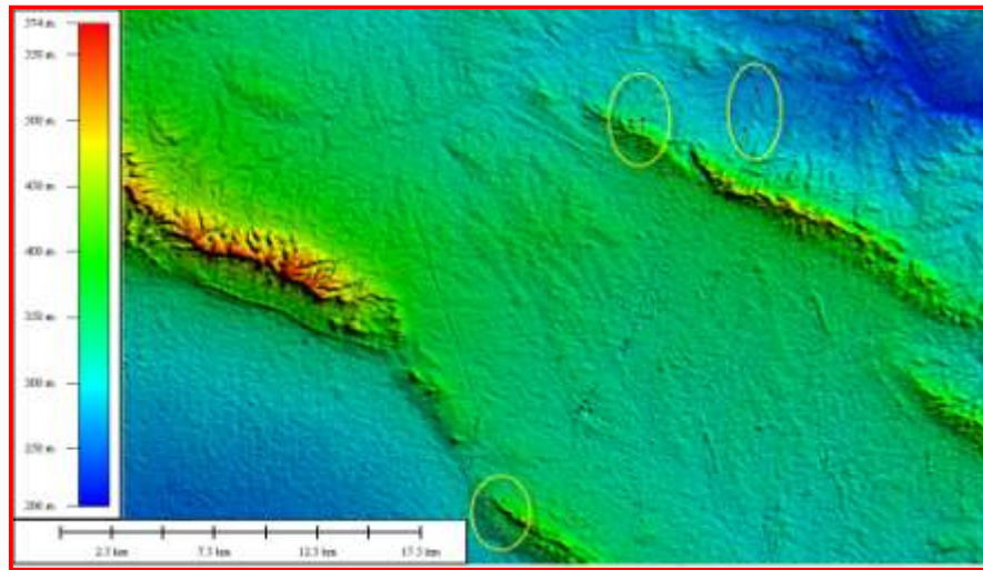
Figure (5): Overlapping of GPS measuring locations with the DEM layer as display by GM10.0 windows
