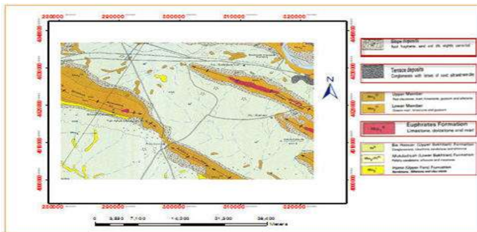
Figure (4): The geological map of the study area (after Varoujan et al, 1995)
