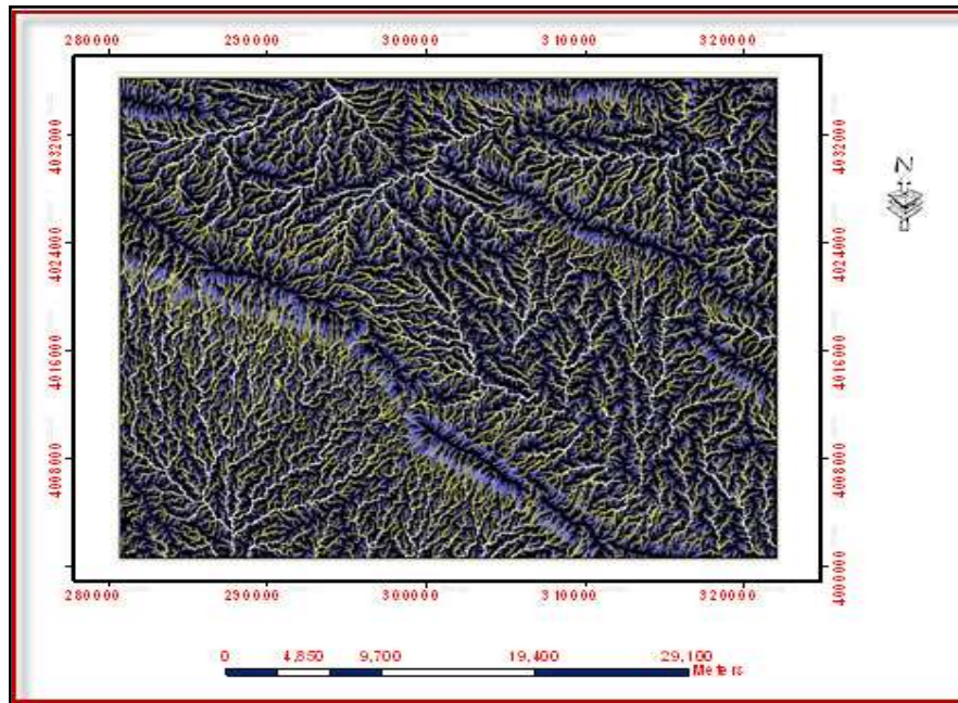
Figure (9): Drainage pattern of the study area
