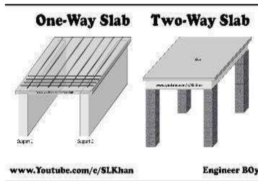
Fig -2: One Way & Two Way Slab
