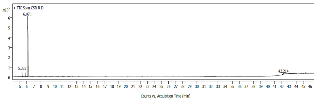
Figure 1: GCMS chromatogram for the aqueous extract of Costusspeciosus rhizome .
