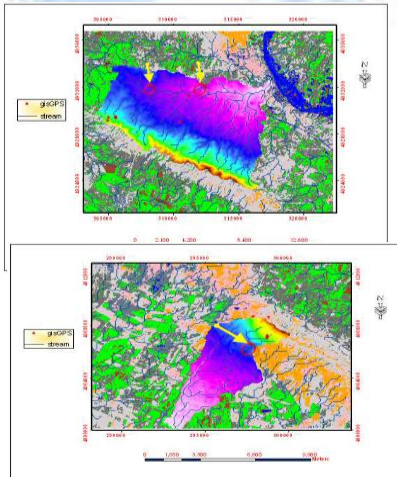
Figure (14): Suggested dam site
