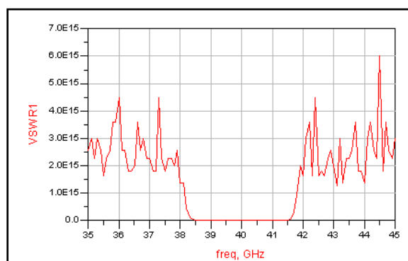
Fig.9 VSWR Vs frequency at 40GHz of BPF
