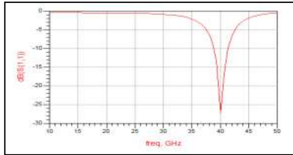
Fig.3 Return loss Vs frequency at 40GHz of LNA
