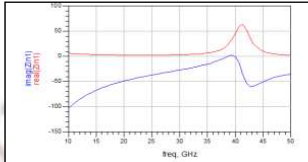
Fig.4 Input impedance variation with frequency of LNA
