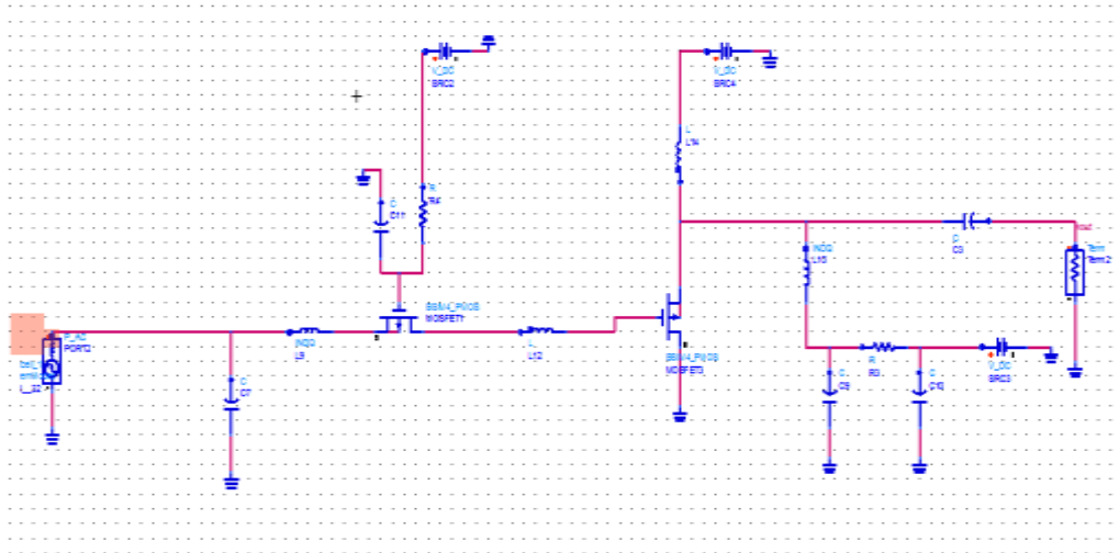
Fig.10 Complete design of receiver system at 40GHz
