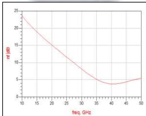
Fig.6 Noise figure Vs frequency of LNA at 40GHz
