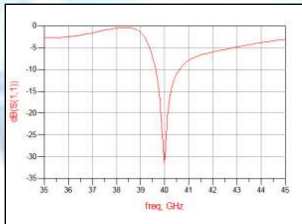
Fig.11 Return loss Vs frequency at 40GHz of receiver system
