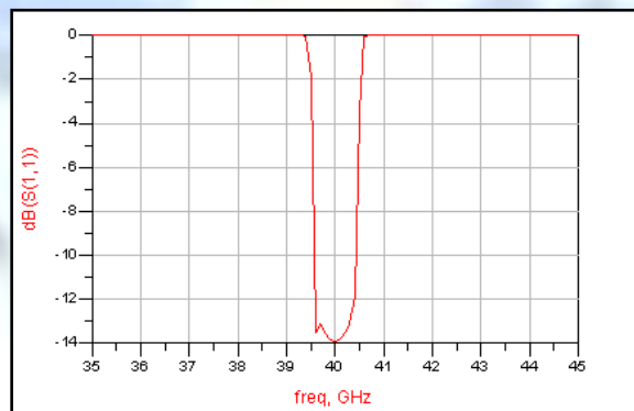
Fig.8 Return loss Vs frequency at 40GHz of filter
