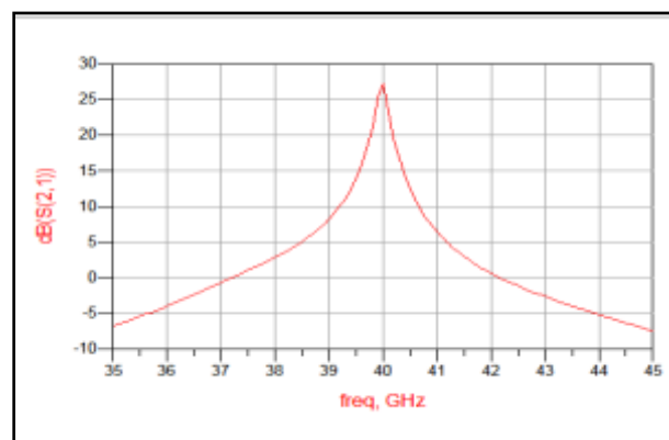
Fig.12 Forward gain Vs frequency at 40GHz
