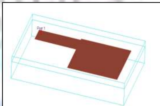
Fig.7 3D view of the designed patch antenna at 40GHz
