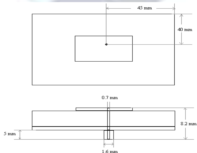
Figure 2.2: Feeding position (Antenna B)
