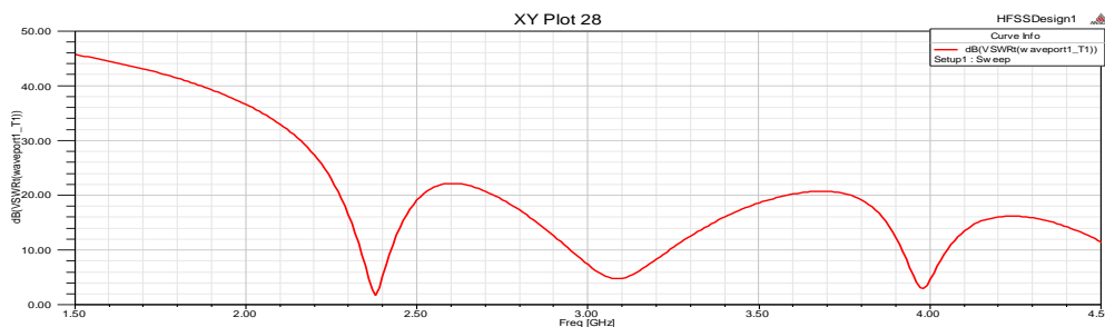
Figure 3.6: VSWR of Patch Antenna (Antenna C)
