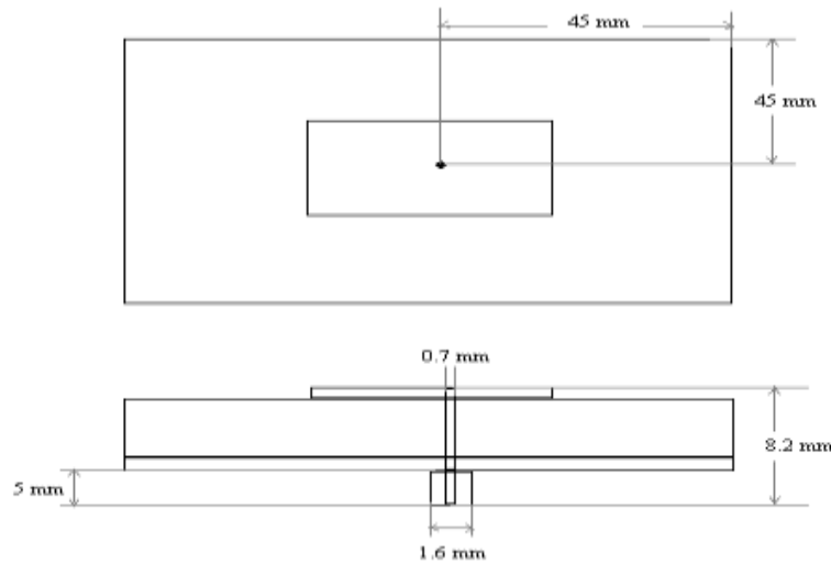
Figure 2.1: Feeding position (Antenna A)
