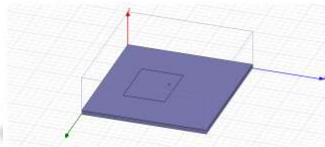
Figure 3.7: Simulation model of patch antenna (Antenna C)
