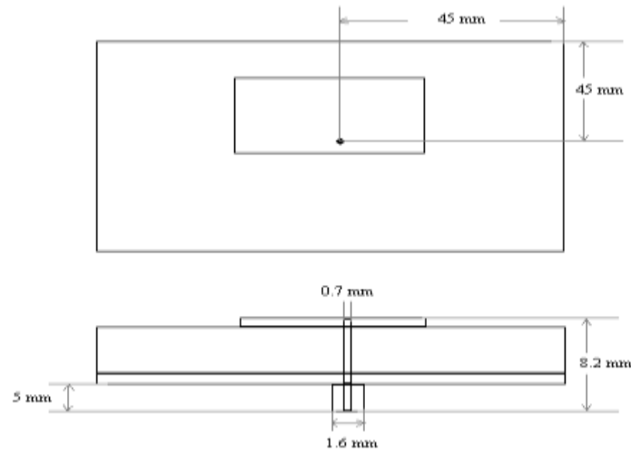
Figure 2.3: Feeding Position (Antenna C)
