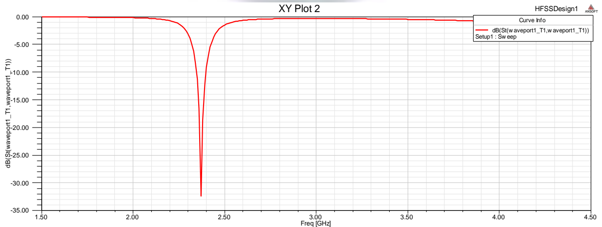
Figure 3.2: Return loss of patch antenna (Antenna A)
