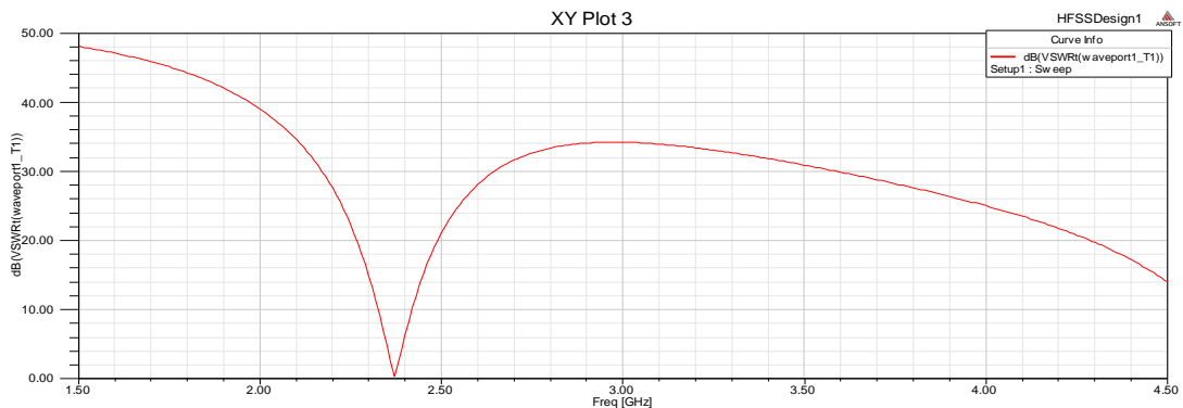
Figure 3.3: VSWR of Patch antenna (Antenna A)
