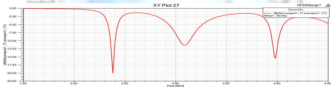
Figure 3.8: Return Loss of patch Antenna (Antenna C)
