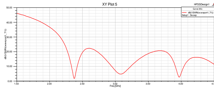
Figure 3.6: VSWR of Patch Antenna (Antenna B)
