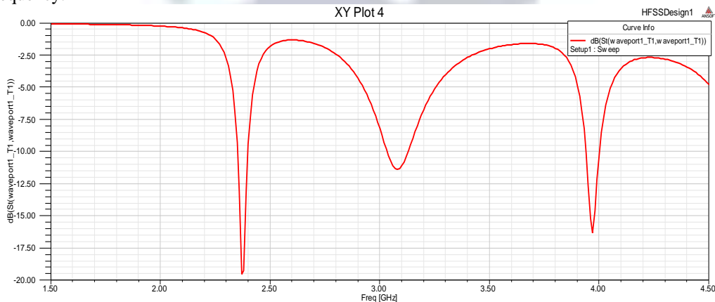
Figure 3.5: Return Loss of patch Antenna (Antenna B)
