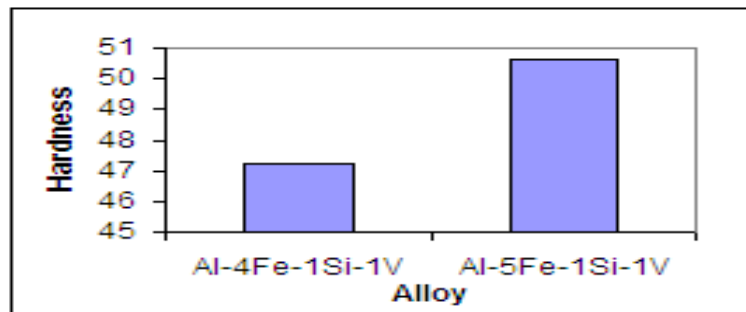
Fig. 2: Hardness of the samples cast in Permanent mould of 12mm dia.
