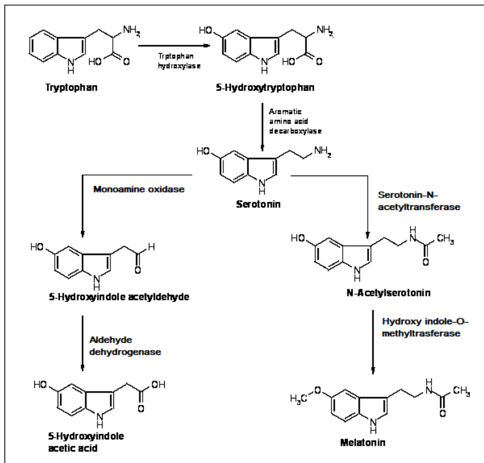
Figure 1: Synthesis of Melatonin
