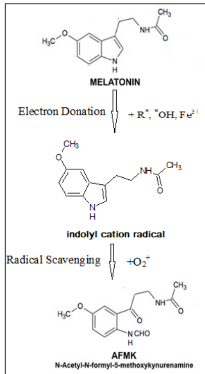
Figure 2: Free-radical scavenging activity of melatonin
