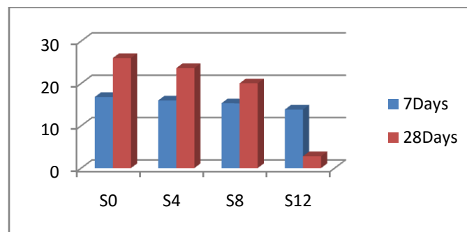
Chart2: Graph showing the variation of tyre rubber versus compressive strength in N/mm2 of M20 grade of concrete
